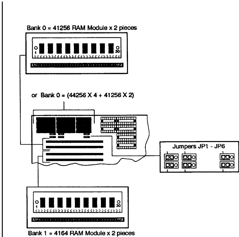
Figure 2-9: 640 KB Total Onboard System Memory
