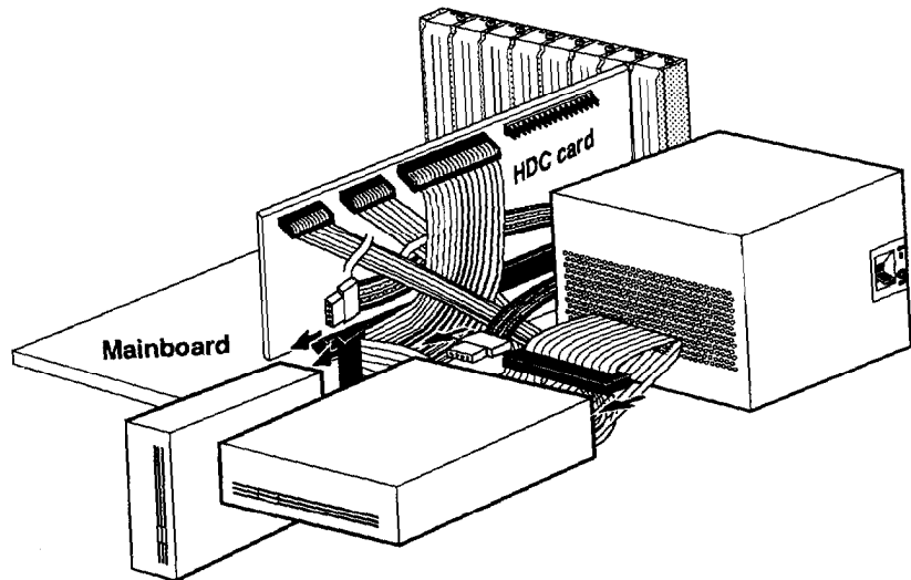
Figure 6-11: Connecting a Hard Disk to an HDC Card
