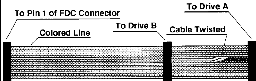
Figure 6-5: Controller Cable for the Floppy Disk Drive
