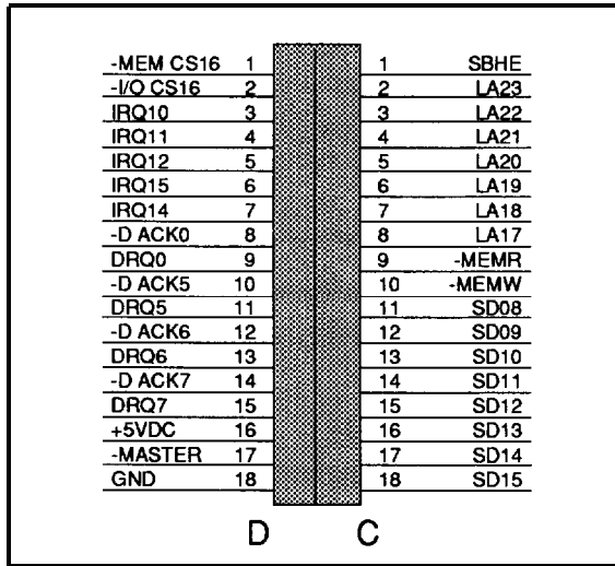
Figure 6-13: 36-Pin Expansion Bus I/O Channels
