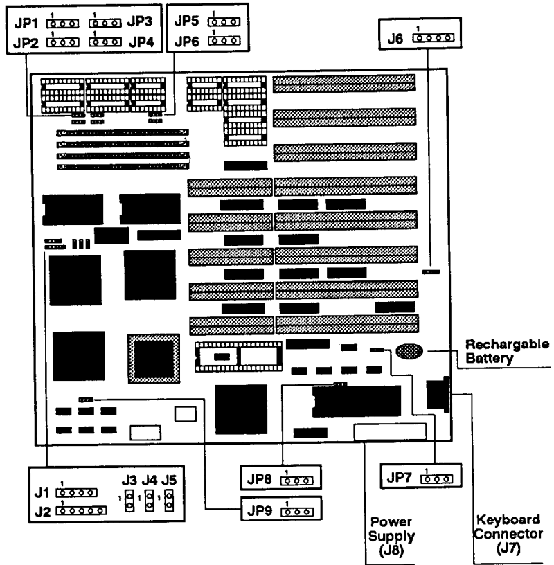
Figure 2-1: Motherboard Layout
