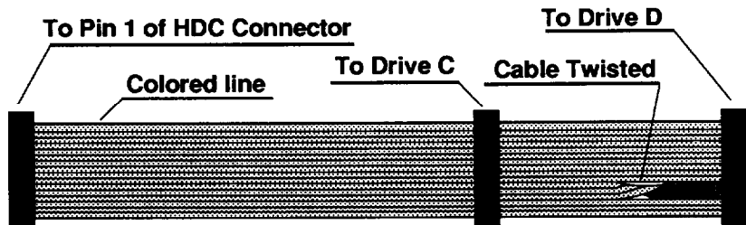
Figure 6-8: Controller Cable for the Hard Disk Drive
