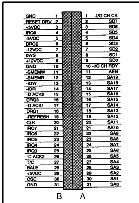
Figure 6-12: 62-Pin Expansion Bus I/O Channels
