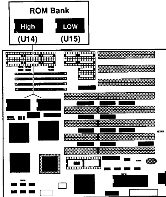
Figure 2-17: Installing ROM
