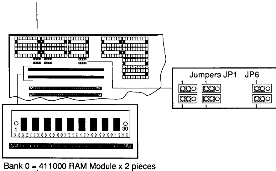
Figure 2-13: 2MB Total Onboard System Memory (B)
