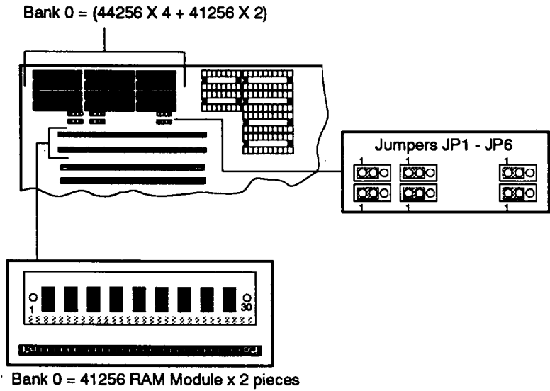
Figure 2-8: 512KB Total Onboard System Memory
