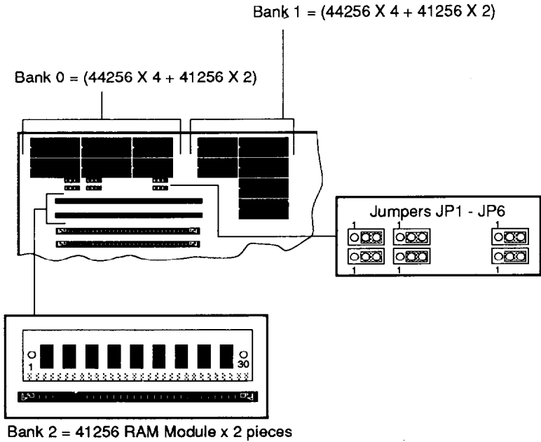
Figure 2-11: 1.5 MB Total Onboard System Memory
