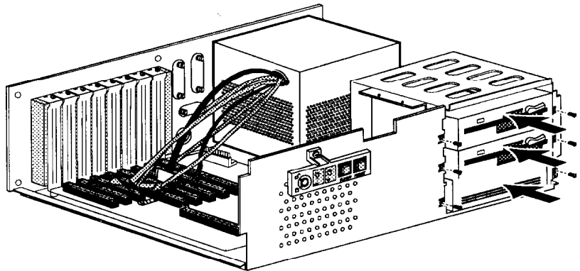
Figure 6-2: Fastening 5.25" Disk Drives
