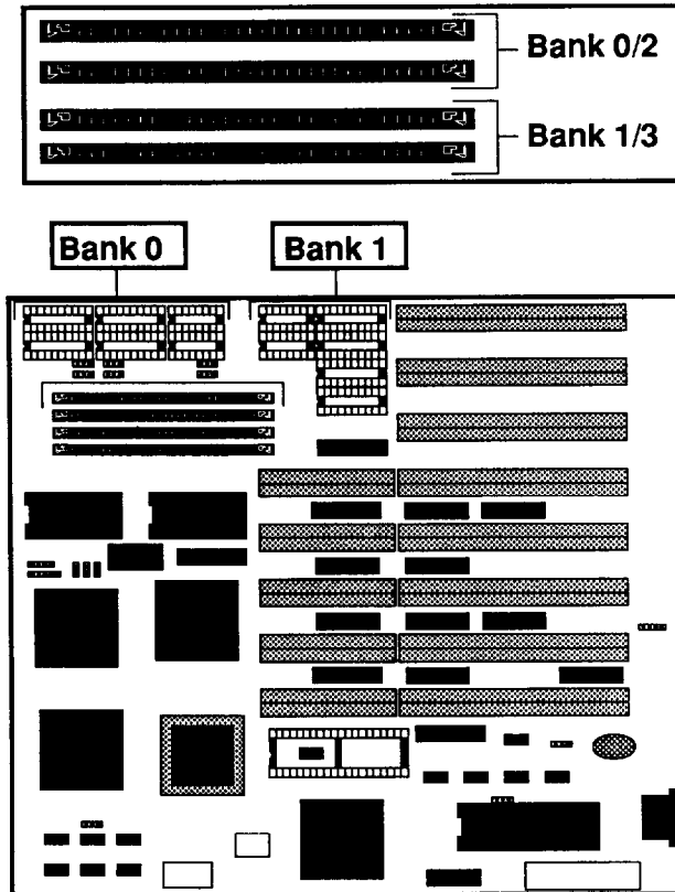
Figure 2-7: RAM Banks
