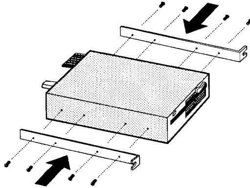
Figure 6-1: Screwing a 5.25" Disk Drive
