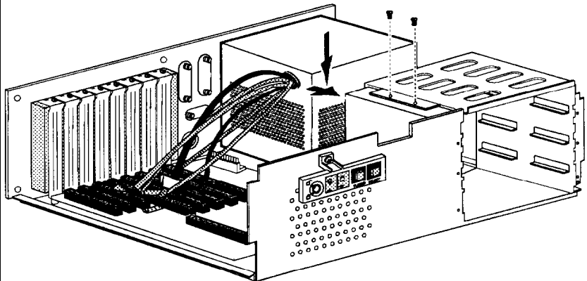
Figure 6-4: Fastening the 3.5" Hard Disk Drive
