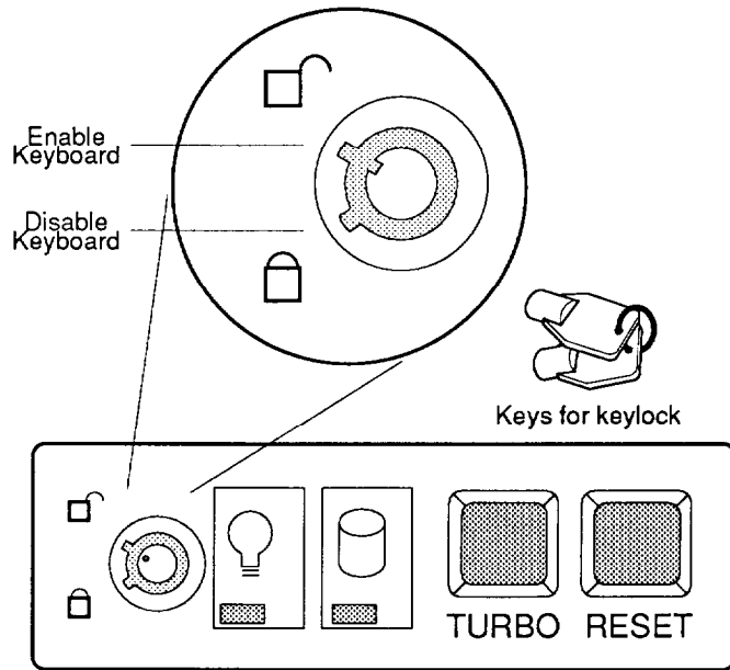
Figure 1-5: Keylock and Two Security-Lock Keys
