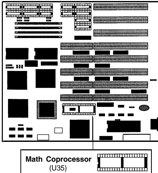
Figure 2-3: The Location of 80287
