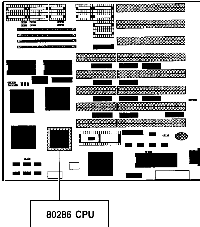
Figure 2-2: The Location of 80286 CPU
