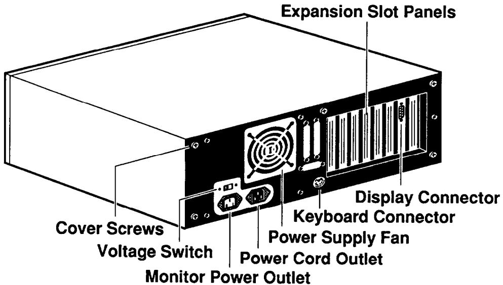
Figure 1-7: Rear Panel
