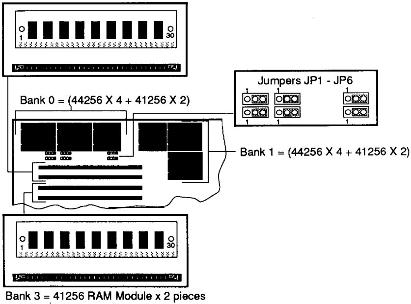
Figure 2-12: 2MB Total Onboard System Memory (A)
