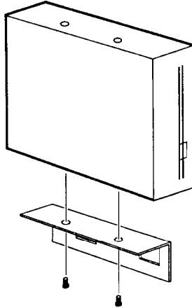
Figure 6-3: Screwing a 3.5" Hard Disk Drive
