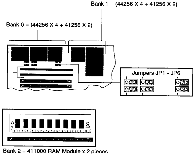
Figure 2-14: 3MB Total Onboard System Memory
